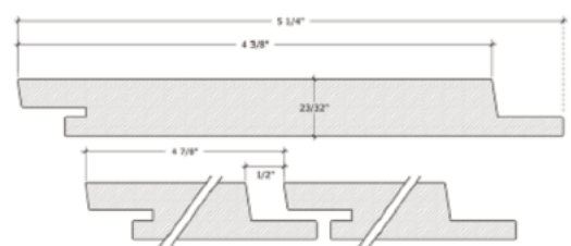
A&BTR CVG 1x6 Nova Rainscreen 1/2" Gap
