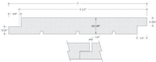
A&BTR CVG Cedar 1X8 Shiplap 1/8" Gap
