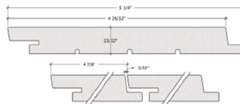
A&BTR CVG 1x6 Nova Rainscreen 3/32" Gap
