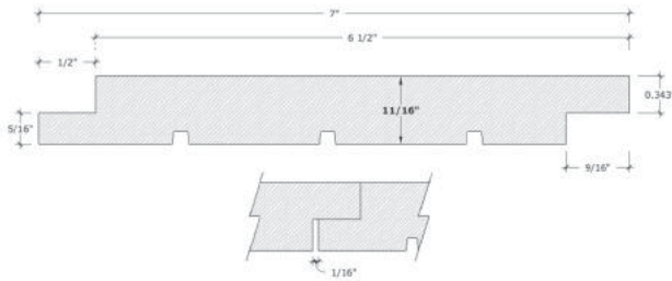
A&BTR CVG Cedar 1X8 Shiplap Tight
