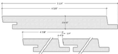
A&BTR CVG 1x6 Nova Rainscreen 1/4" Gap
